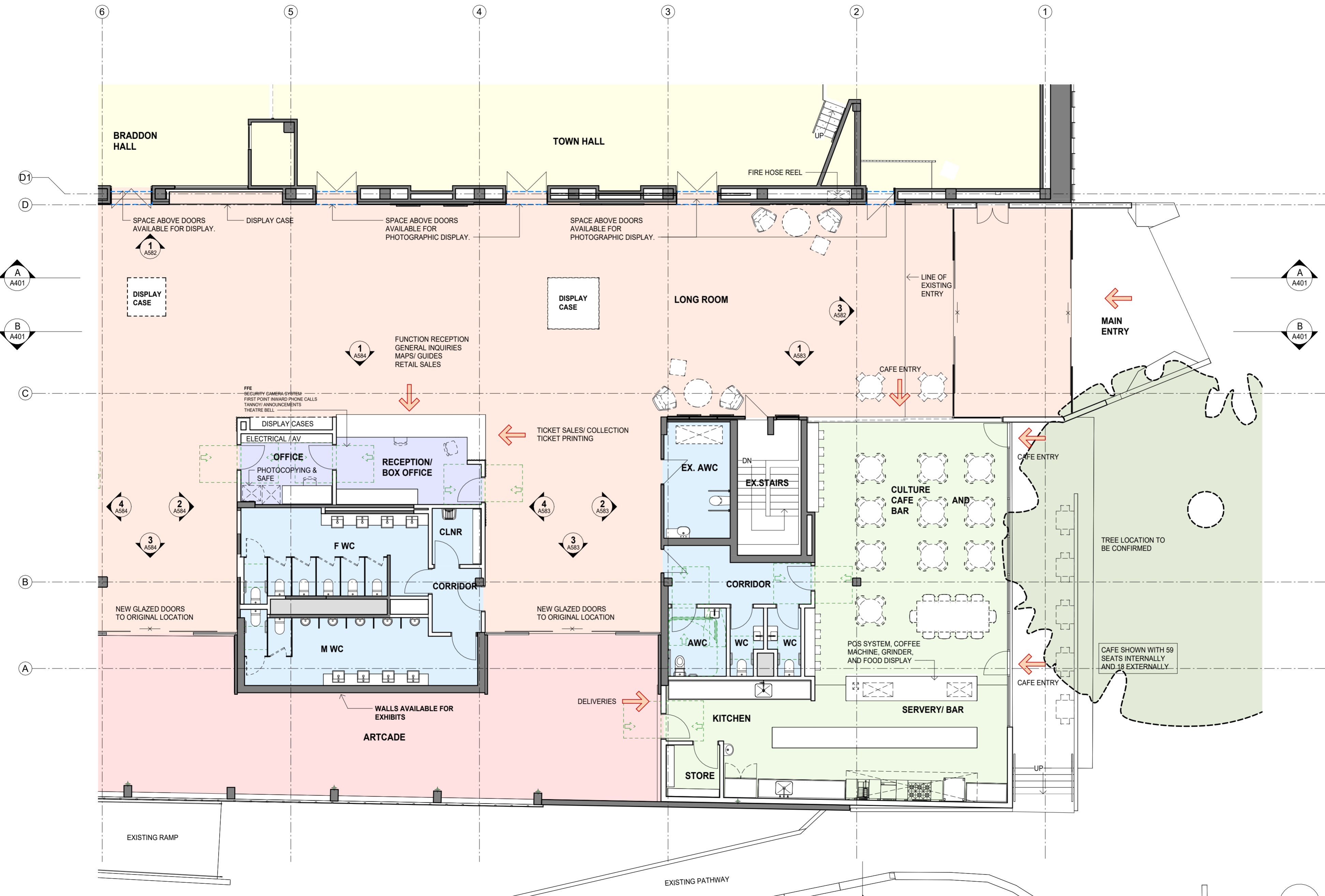
1 GROUND FLOOR (SOUTH) 1 : 100
