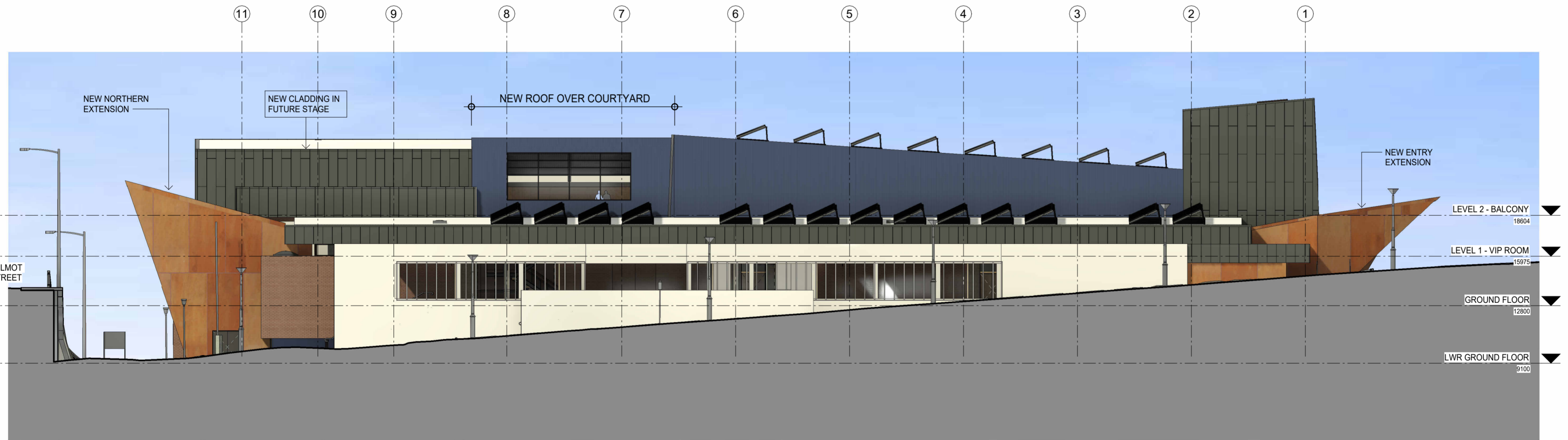
2 WESTERN ELEVATION (CAR PARK) 1 : 200
