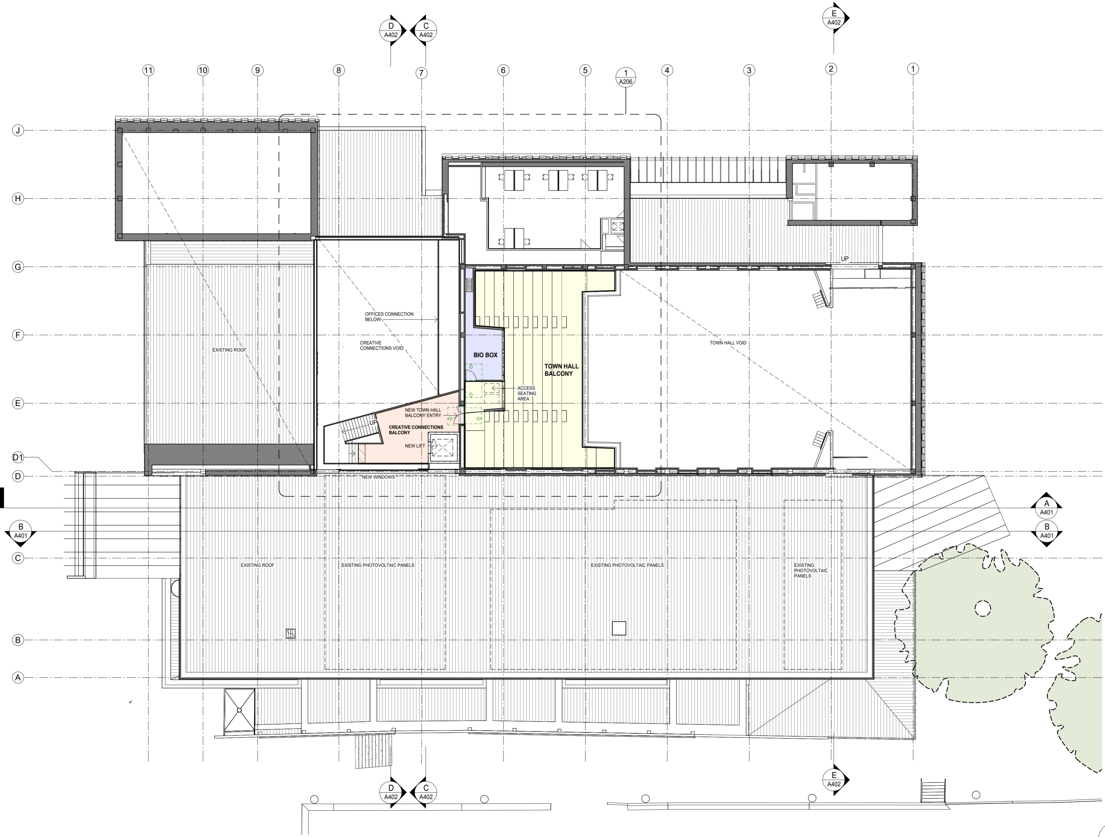
1 LEVEL 2 - BALCONY 1:200
