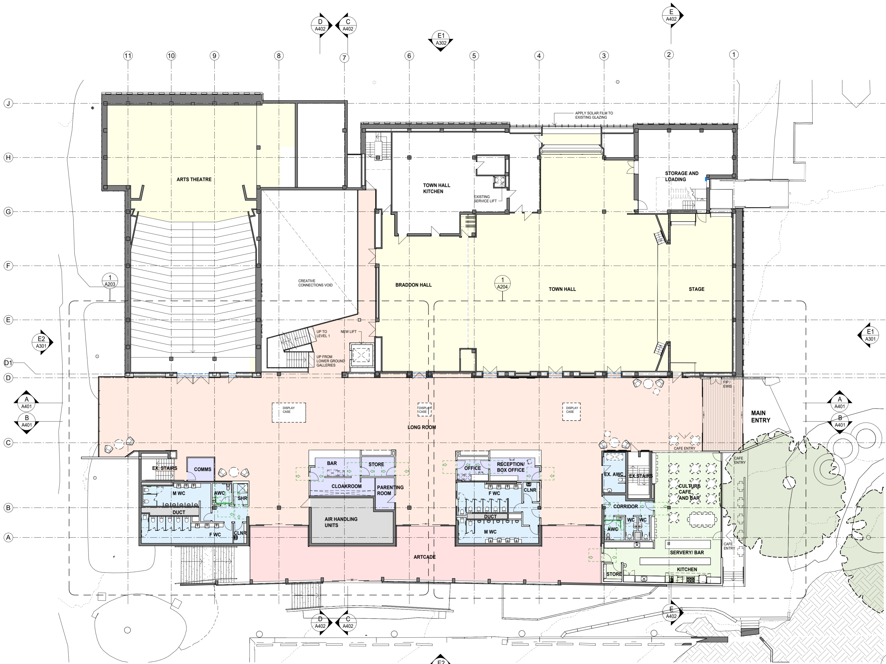
B GROUND FLOOR PLAN 1 : 200
